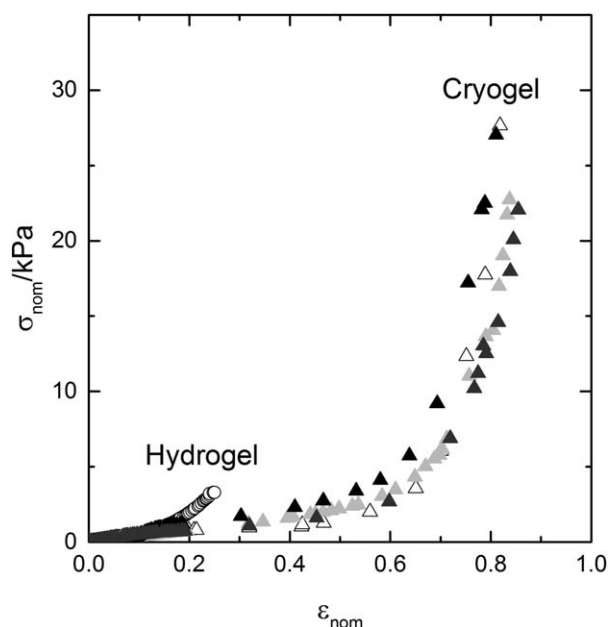
Figure 3. Stress–strain curves of HA cryogels (triangles) and HA hydrogel (circle) formed at 7.3% HA. T_{\text{prep}} = -18^{\circ}\text{C} . C_{\text{EGDE}} 0.9% (open triangle), 1.7% (light gray), 2% (black), and 2.5% dark gray. The reference HA hydrogel was prepared at T_{\text{prep}} = 20^{\circ}\text{C} and C_{\text{EGDE}} = 2.5\% .
